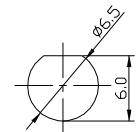
RECOMMENDED SMA MOUNTING HOLE
